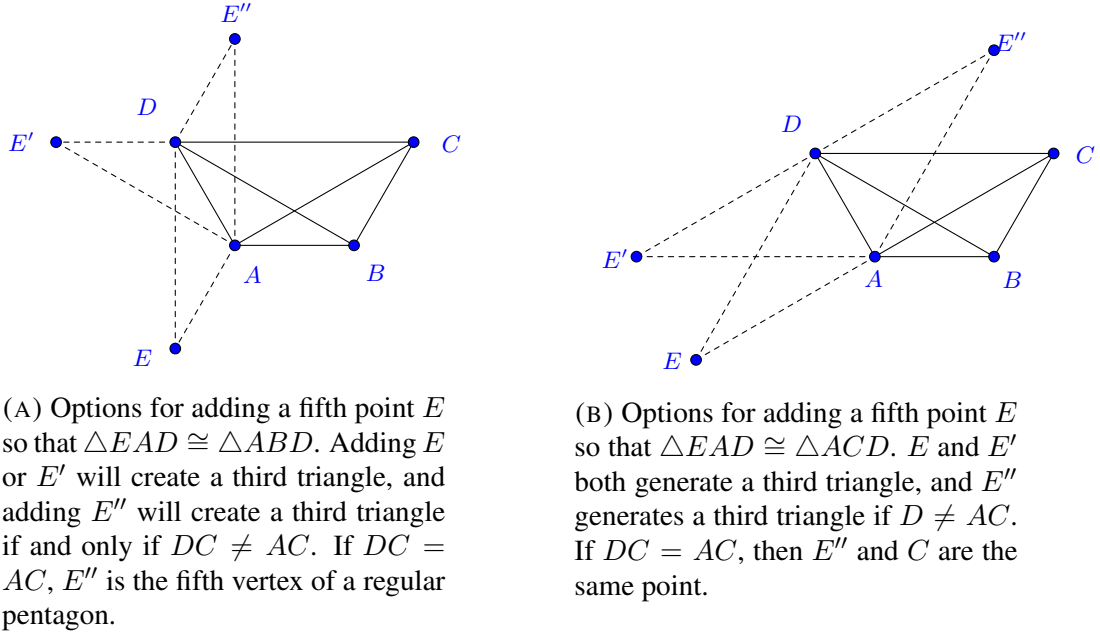
FIGURE 8. Possible additions of a fifth point when three sides are congruent.
