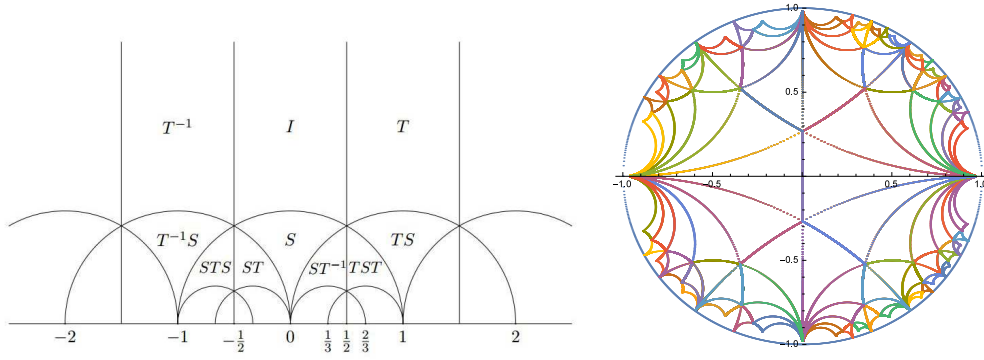
FIGURE 1. Plot of tessellation of the upper half plane (or unit disk) by the fundamental domain of SL_2(\mathbb{Z}) , where T sends z to z + 1 and S sends z to -1/z .
