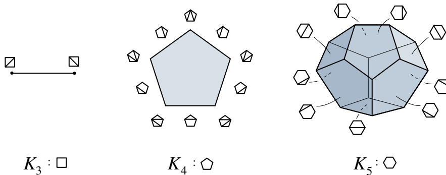
FIGURE 2. Associahedra K_3 , K_4 and K_5
