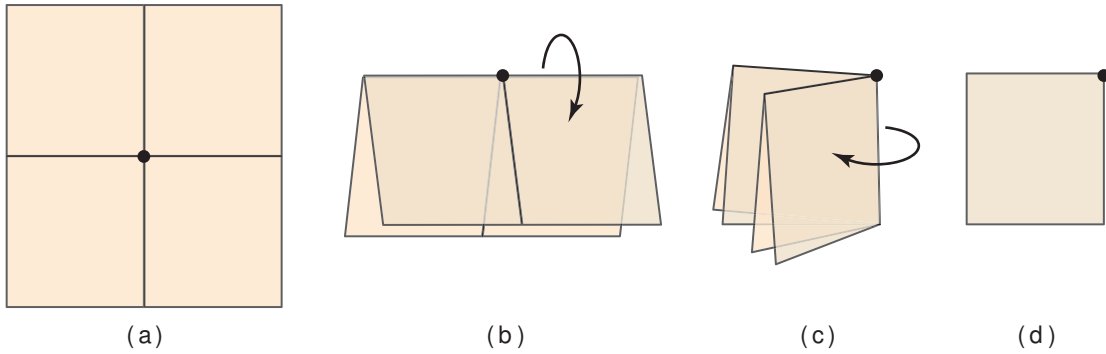
FIGURE 13. The 2^{n-2} : 1 folding of cubes.
