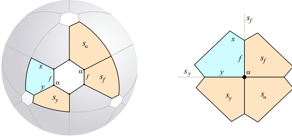
FIGURE 8. Reflections locally around \mathcal{C}(A_3)_\# .
