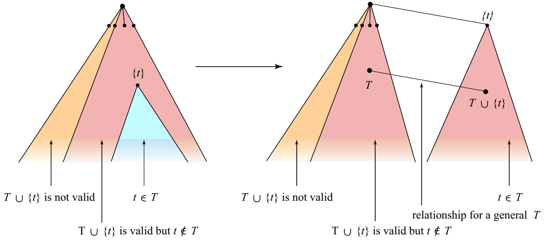
FIGURE 5. A sketch of the poset lattice before and after promotion of tube \{t\} . Regions shaded with like colors are isomorphic as posets.
