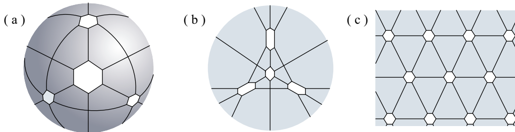
FIGURE 7. Minimal blow-ups of (a) \mathcal{C}A_3 , (b) \mathbb{P}\mathcal{C}(A_3) and (c) \mathcal{C}\tilde{A}_2 .
