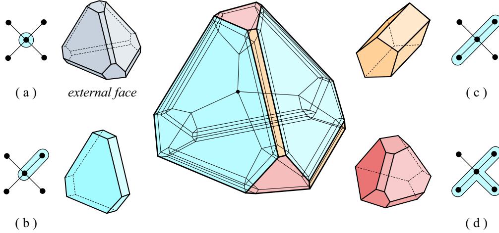
FIGURE 4. The Schlegel diagrams of a 4-polytope along with its four types of facets.
