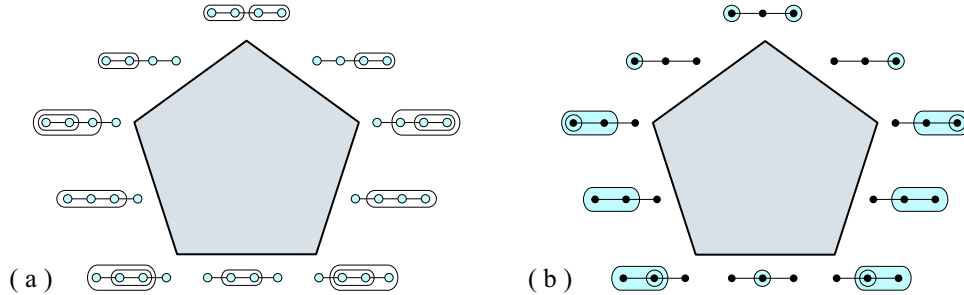
FIGURE 1. Associahedron K_4 labeled with (a) bracketings and (b) tubings.
