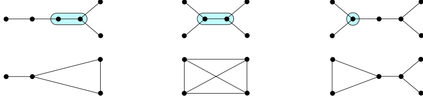
FIGURE 3. Examples of 1-tubings and their reconnected complements.
