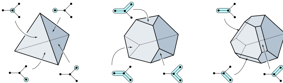
FIGURE 2. Iterated truncations of the 3-simplex based on an underlying graph.
