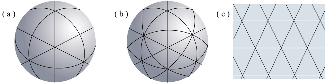
FIGURE 6. Coxeter complexes \mathcal{C}A_3 , \mathcal{C}B_3 , and \mathcal{C}\tilde{A}_2 .
