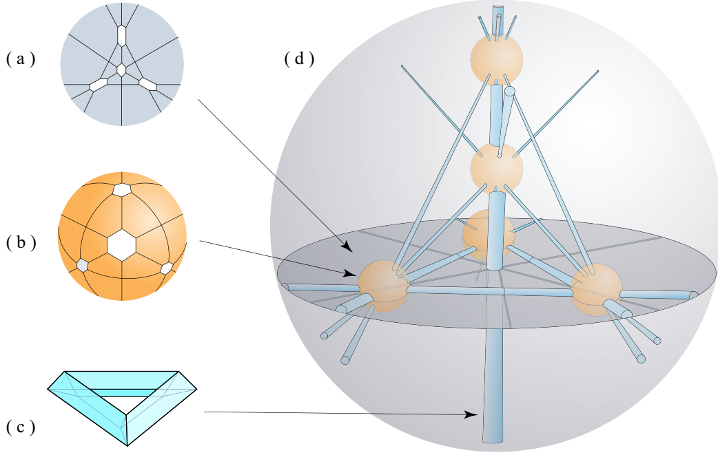
FIGURE 9. The projective Coxeter complex (d) \mathbb{P}\mathcal{C}(A_4)_\# along with components (a) \mathbb{P}\mathcal{C}(A_3)_\# , (b) \mathcal{C}(A_3)_\# and (c) \mathbb{P}\mathcal{C}(A_2)_\# \times \mathbb{P}\mathcal{C}(A_2)_\# .
