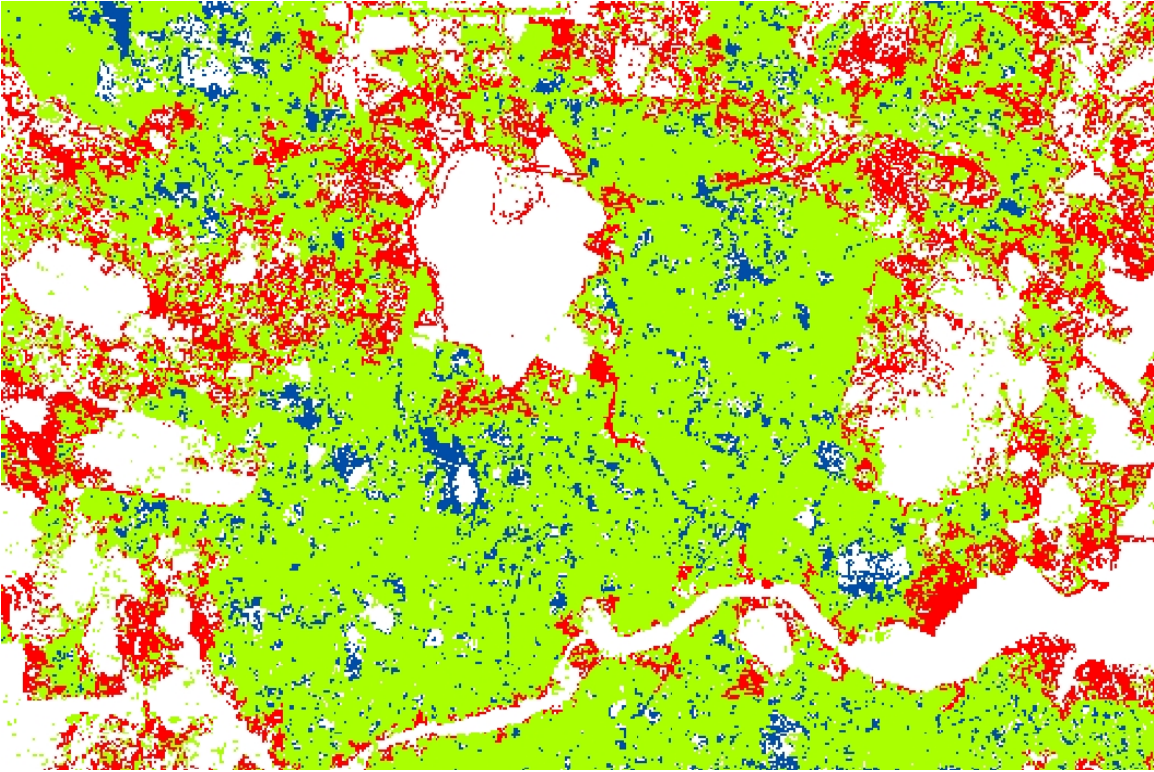
Figure 2: Classification of Urban Land Cover in Hyderabad, India
