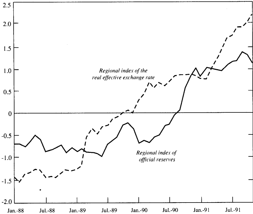
Figure 7. First Principal Components, January 1988–December 1991
