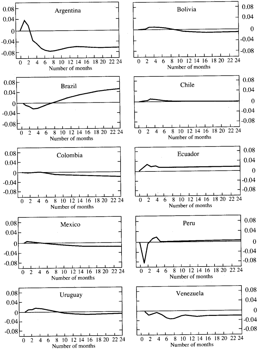
Figure 10. Response of the Real Exchange Rate to a One-Standard-Deviation in the First Foreign Factor
