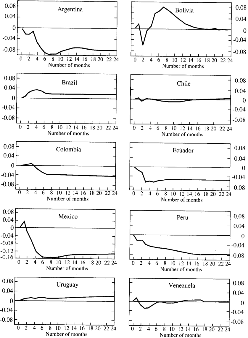
Figure 9. Response of Official Reserves to a One-Standard-Deviation Shock in the First Foreign Factor
