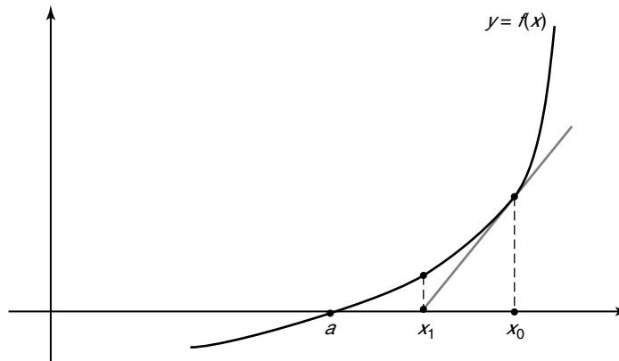
Figure 1.1 Newton's Method
