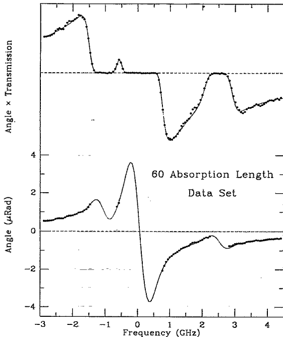
FIG. 3. Combined parity rotation data from the data set at 60 absorption lengths, representing 40 h of data acquisition. The top trace shows (angle) \times (transmission) data, as measured and analyzed in the experiment. Below is the same data with the transmission envelope divided out to show the dispersive shape of the pure PNC rotation. Points with very large angle uncertainty, due to near zero light transmission, are omitted. Solid lines represent fitted theoretical profiles.
