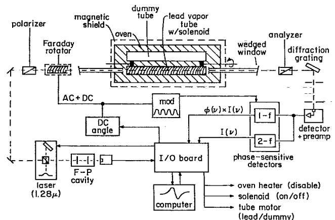
FIG. 1. Block diagram of the experiment.
